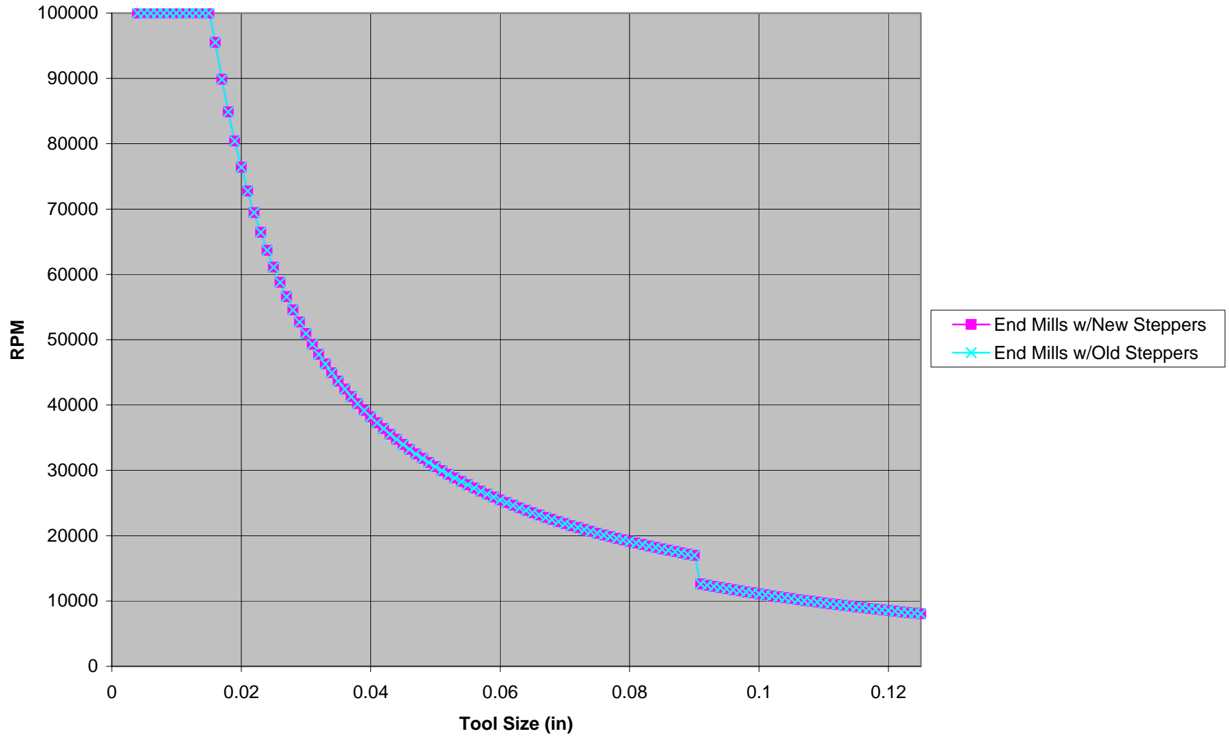
RPM vs Tool Size
